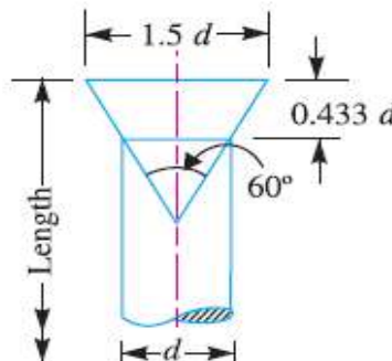
(f) Flat counter sunk head 60°.
