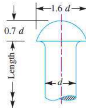
(a) Snap head.
