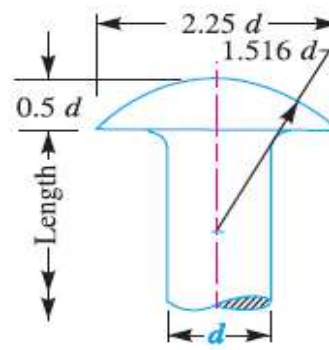
(c) Mushroom head.
