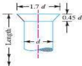
(g) Counter-sunk head.
