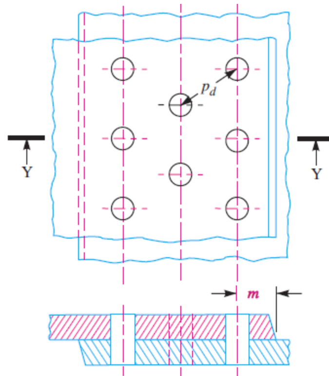
(b) Zig-zag riveting. Activate 1
