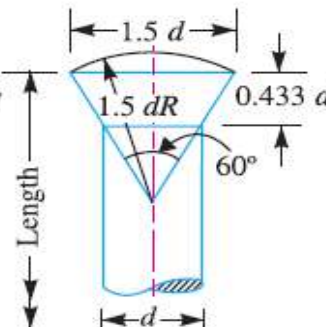
(g) Round counter sunk head 60°.
