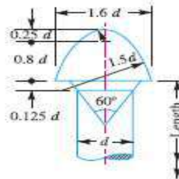
(f) Conical head.
