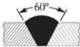
(b) Single V-butt joint.
